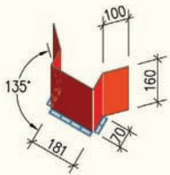
WFP SEALING ELEMENT CORNER FB
