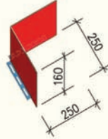
WFP SEALING ELEMENT CORNER 90°
