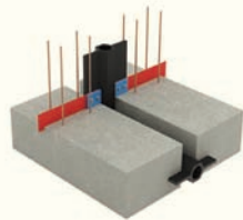
WFP EXPANSION JOINT CONNECTION
